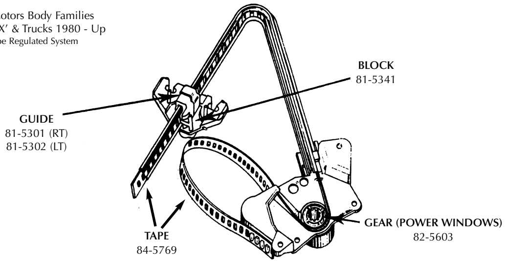
(ILLUSTRATION POWER WINDOW REGULATOR)
