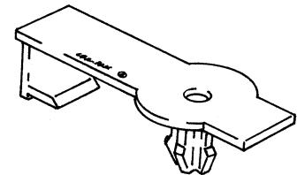
99-8065 Replaces: 5008055AA GROMMET-WINDOW TO REGULATOR Plastic Hole: M12.7, Glass Thickness 3.5MM Screw M6.3 Chrysler Neon 2000 UNIT PACKAGE 15
