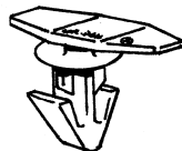
98-7846 Replaces: 10283414, 10405030 CLIP-WEATHERSTRIP Front & Rear Doors Plastic G.M. "W" Body '97/ UNIT PACKAGE 50
