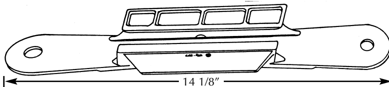
88-6468 Replaces: 4396736 LIFT-CHANNEL DOOR GLASS FRONT DOOR Plastic Chrysler Products, Shadow, Sundance 2 Door '87 UNIT PACKAGE 1
