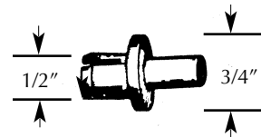
B-7733 Replaces: 6023695 RIVET-TAILGATE GLASS CHANNEL Plastic Plymouth, Dodge '63 UNIT PACKAGE 100
